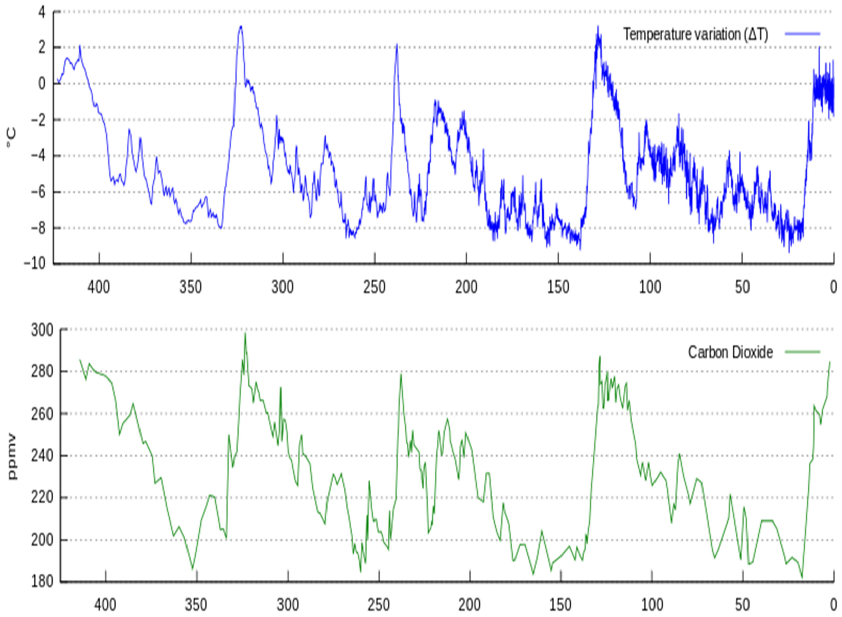
CHART 9 – CO 2 fluctuations past 400K years.
